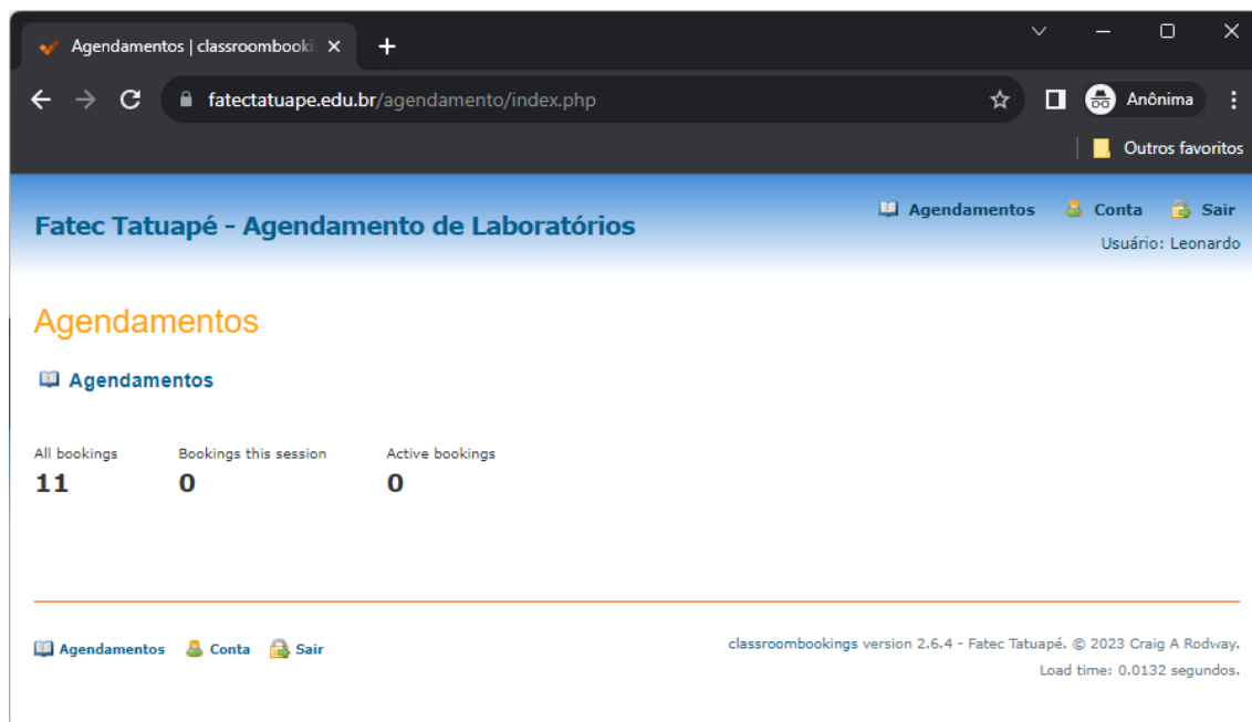
Fig.2 – Tela inicial
