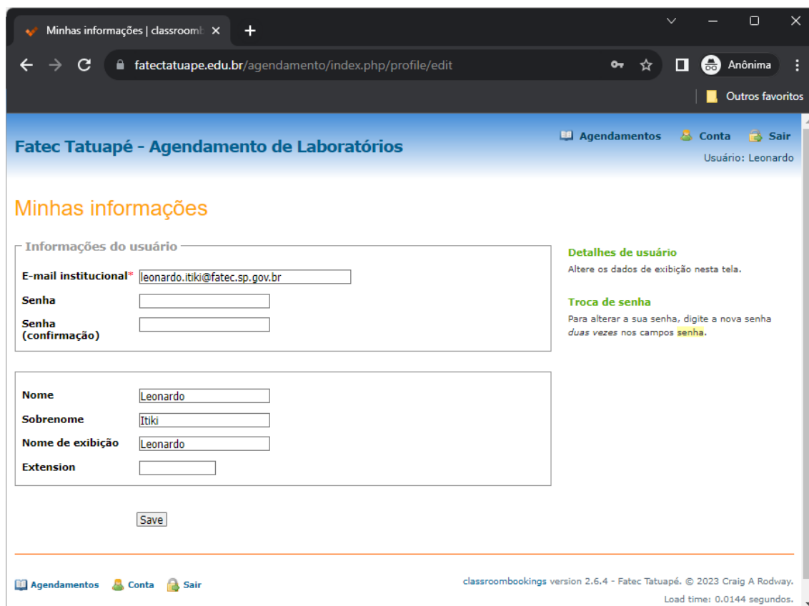
Fig.3 – Tela Account .
